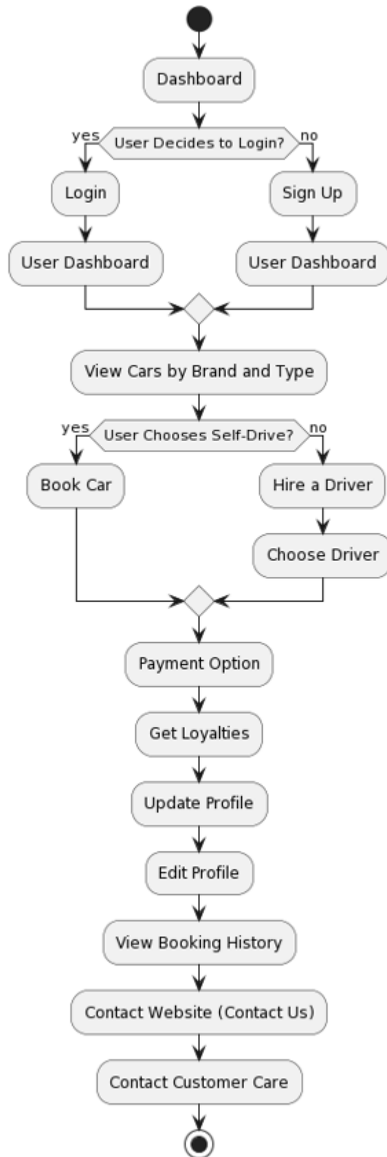
Figure 10 Activity Diagram (User Functions)
