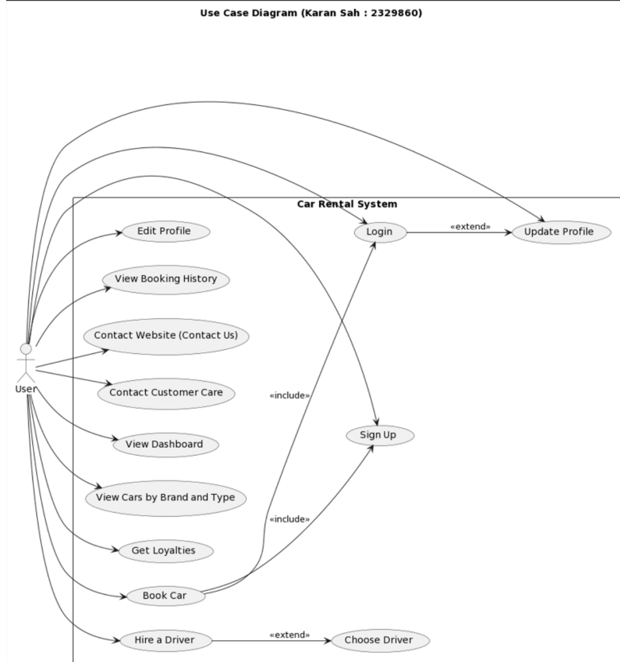
Figure 7 Use Case Diagram (User Side)
