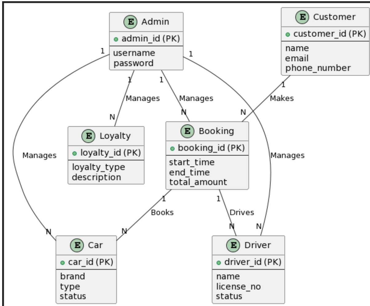
Figure 12 Entity Relationship Diagram
